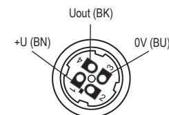
Inside of the connector socket (variant "C")
