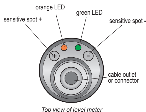
Top view of level meter
