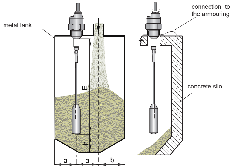
Installation of level meter with rope electrode
