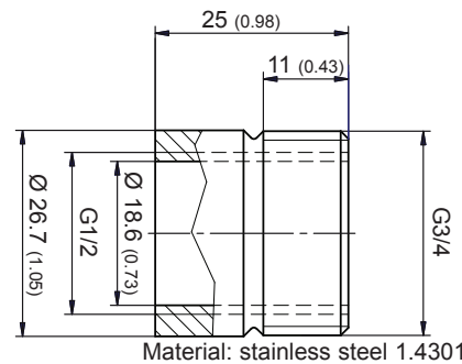
HA074001 Welding nipple
