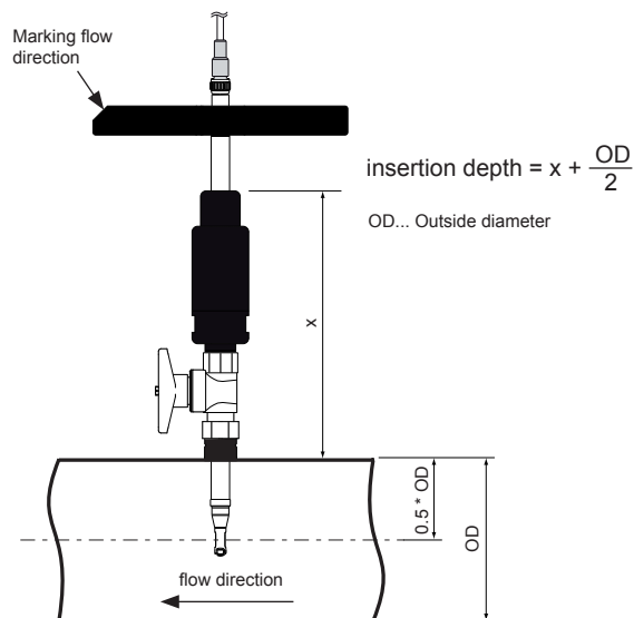
EE776 Assembly - insertion depth
