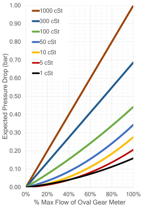
Oval Gear Pressure Drop Information
