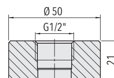
Welding flange for G1/2" (1.4301) Ordering No. C27804
