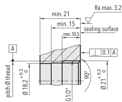
Mounting thread G1/2" DIN EN ISO 1179-1
