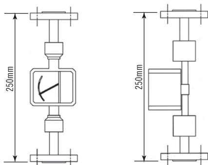
MF200-T Metal Tube Flow Meter Flange Model: Flange Connection
