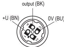
Fig. 4: Inside of the connector socket
