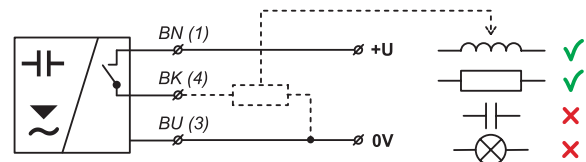
Fig. 2: PNP output type sensor connection (configuration N, NT, Xd)
