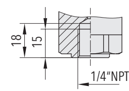
1/4" NPT female
