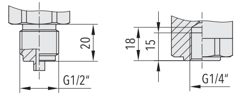
G1/2" male
