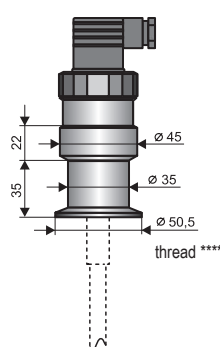
Housing with Tri-clamp coupling
