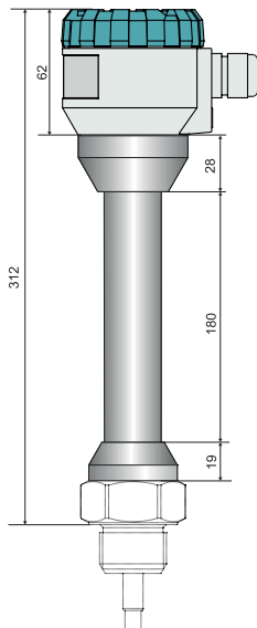
High temperature performance CLM-70_T**
