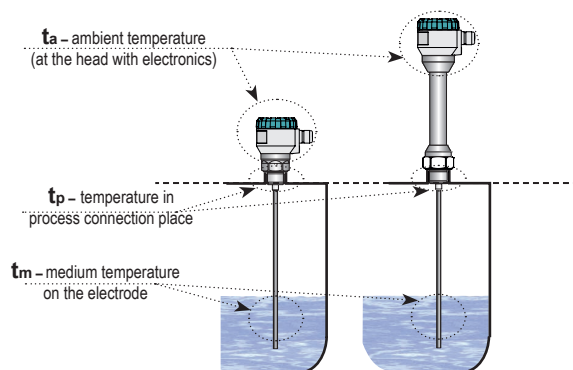
Fig. 1: Illustration of temperature measurement areas
