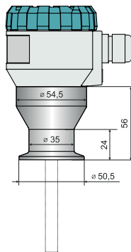
Process connection Tri-clamp***
