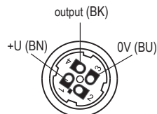
Fig. 4: Inside of the connector socket
