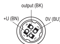
Inside of the connector socket
