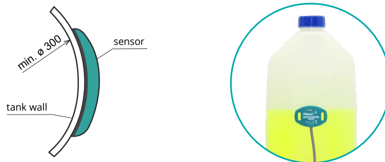
Fastening the FLD-32 using self-adhesive layer
