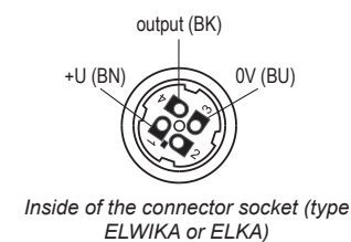
NAMUR type sensors connection (variants Xi and XiM)
