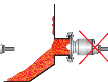
Correct and incorrect installation with a long tube for process connection with Tri-Clamp
