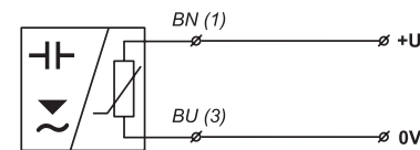
NAMUR type sensors connection (variants Xi and XiM)
